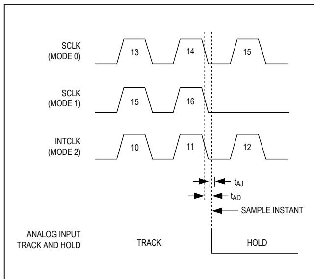
Figure 21. Aperture Diagram
