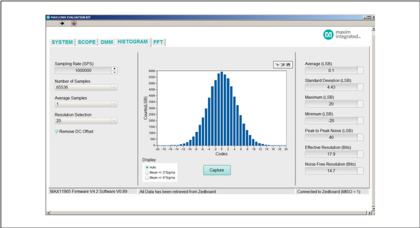
Figure 11. MAX11905 Output Data Histogram (Inputs Shorted, Averaging = 1, f_{SAMPLE} = 1\text{Mps} )
