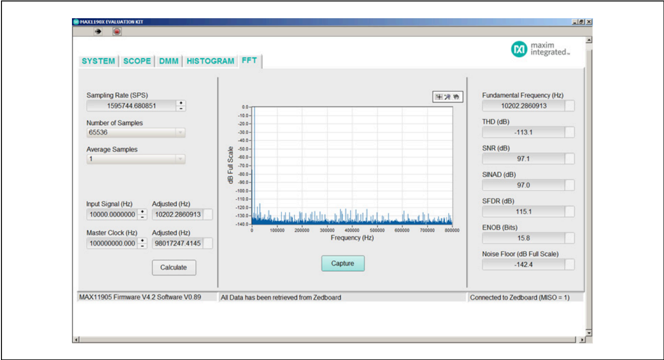
Figure 10. MAX11905 FFT ( f_{SAMPLE} = 1.6\text{Mps} , f_{IN} = 10\text{kHz} )
