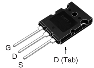
TO-264 (IXFK)
