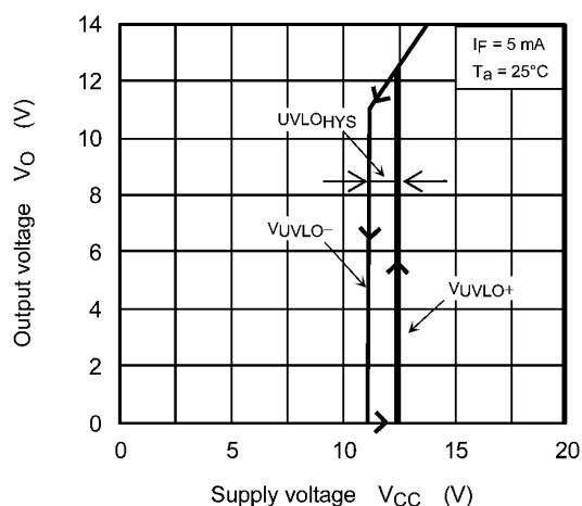
Fig. 12.2.12 V_O(V_{VLO}) - V_{CC}
