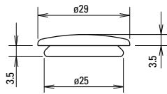
HW-VU1 Dual Pushbutton Barrier
