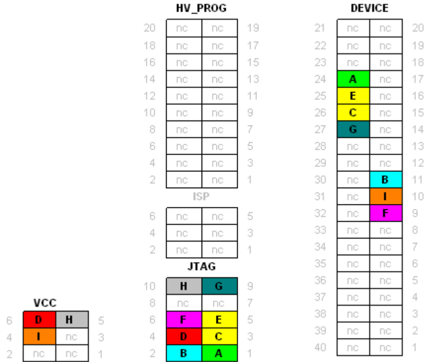
Figure 6-3. Parallel Programming
