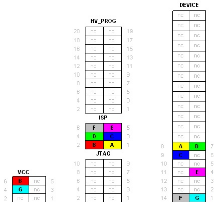
Figure 6-13. SPI Programming and debugWIRE Debugging
