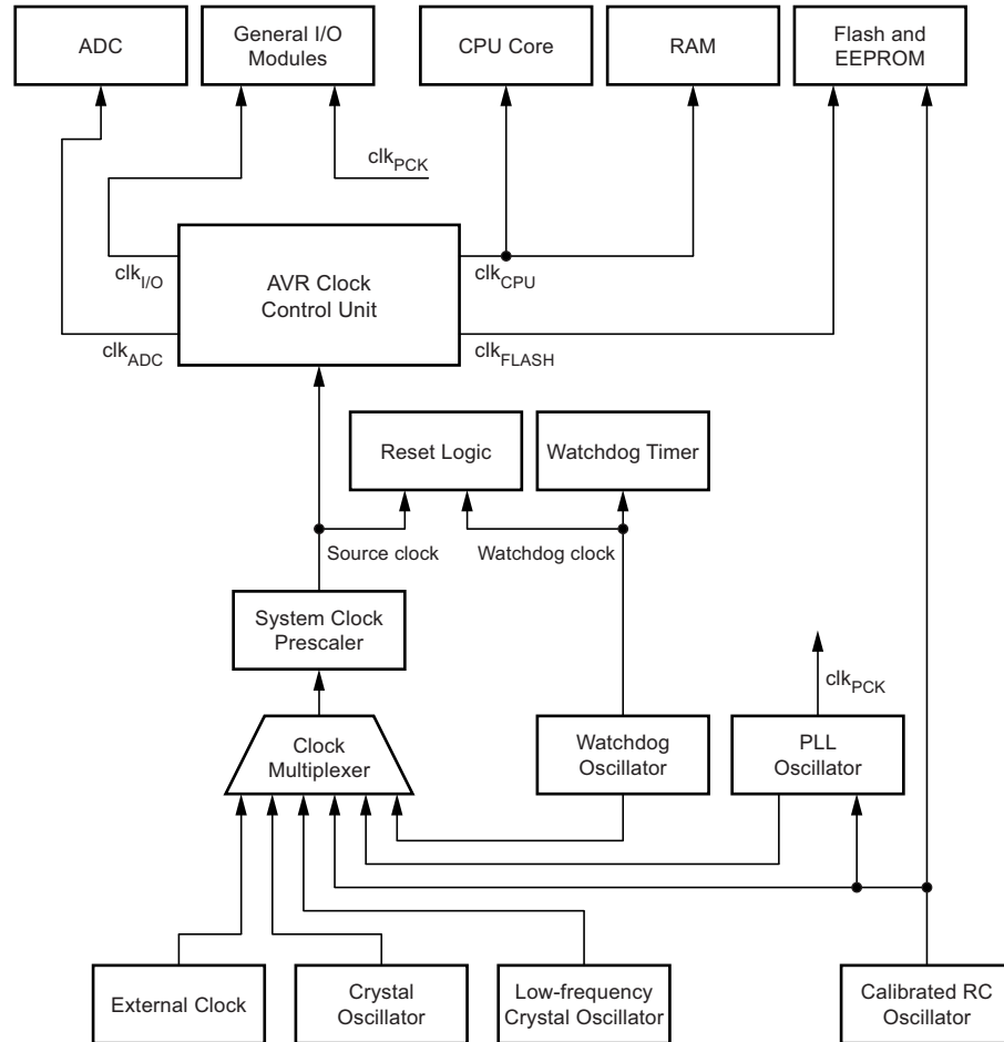
Figure 5-1. Clock Distribution
