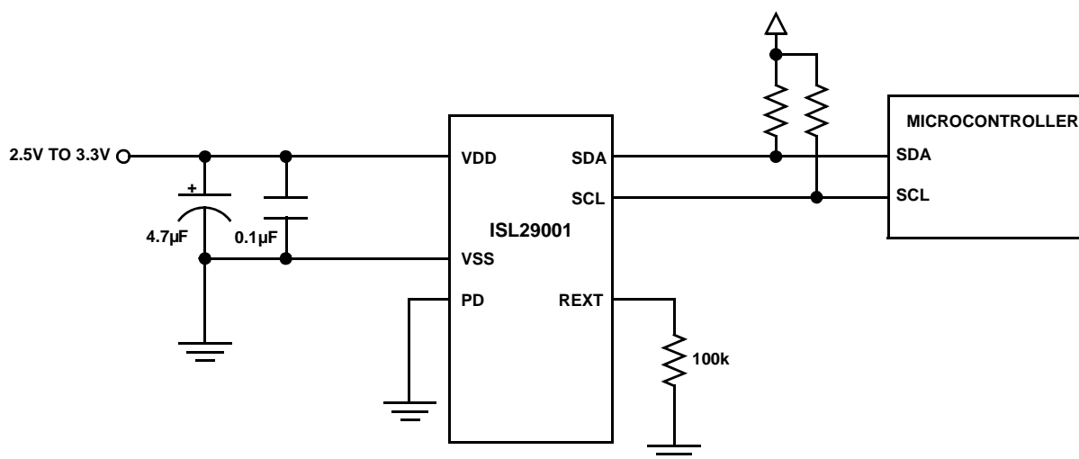
FIGURE 14. TYPICAL CIRCUIT
