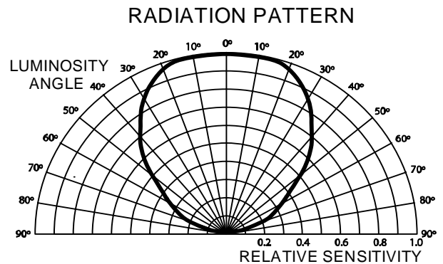
FIGURE 13. RADIATION PATTERN
