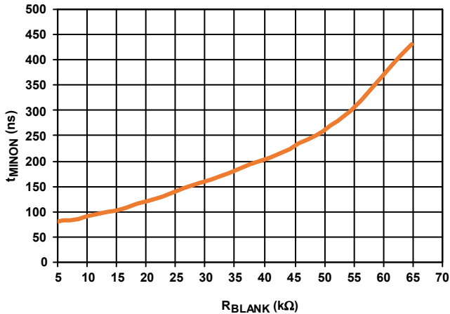
FIGURE 57. t_{\text{MINON}} vs R_{\text{BLANK}}
