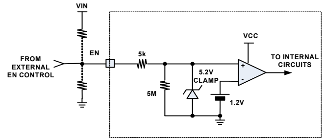
FIGURE 59. ENABLE BLOCK
