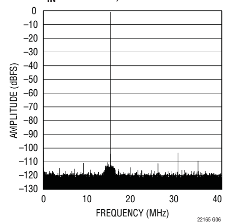
LTC2216 64k Point FFT, f_{IN} = 15.1\text{MHz} , -1\text{dBFS}
