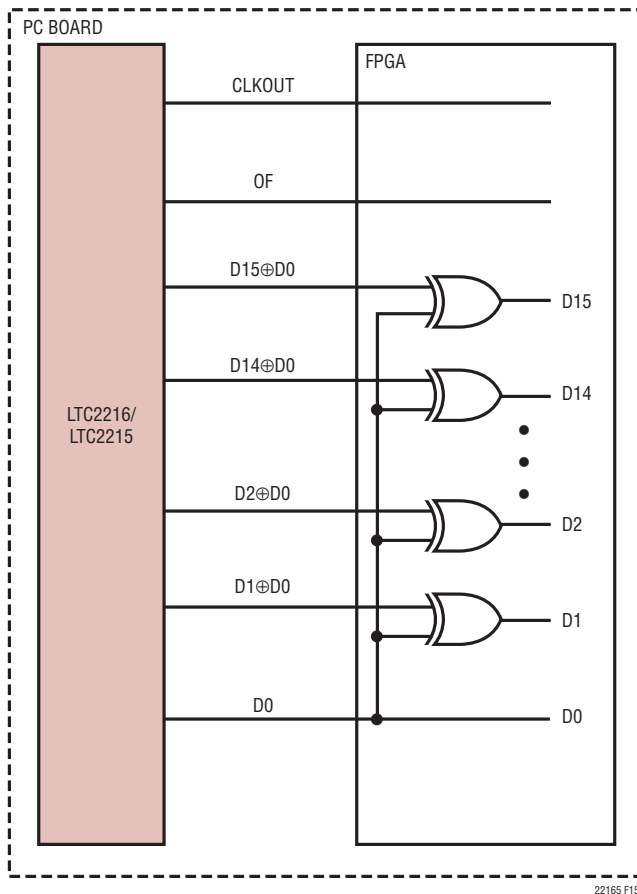
Figure 15. Descrambling a Scrambled Digital Output
