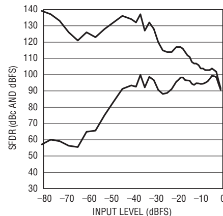
SFDR vs Input Level, f_{IN} = 70.5\text{MHz} , Dither "On"
