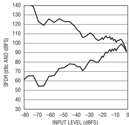
SFDR vs Input Level, f_{IN} = 70.5\text{MHz} , Dither "Off"
