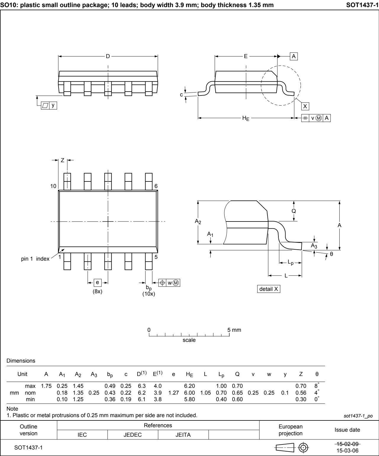
Figure 7. Package outline SOT108-1 (SO10)
