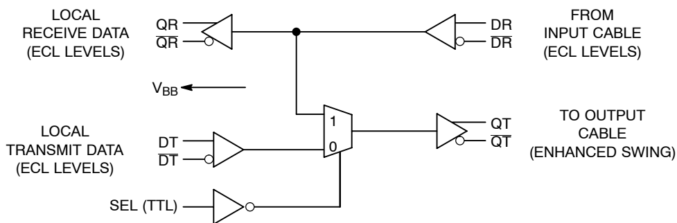
Figure 2. Logic Diagram
