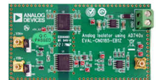
CN0185 circuit evaluation board.
