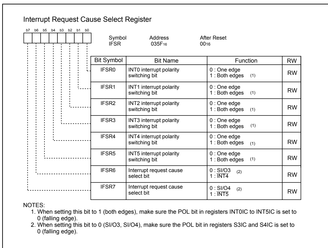
Figure 9.11 IFSR Register
