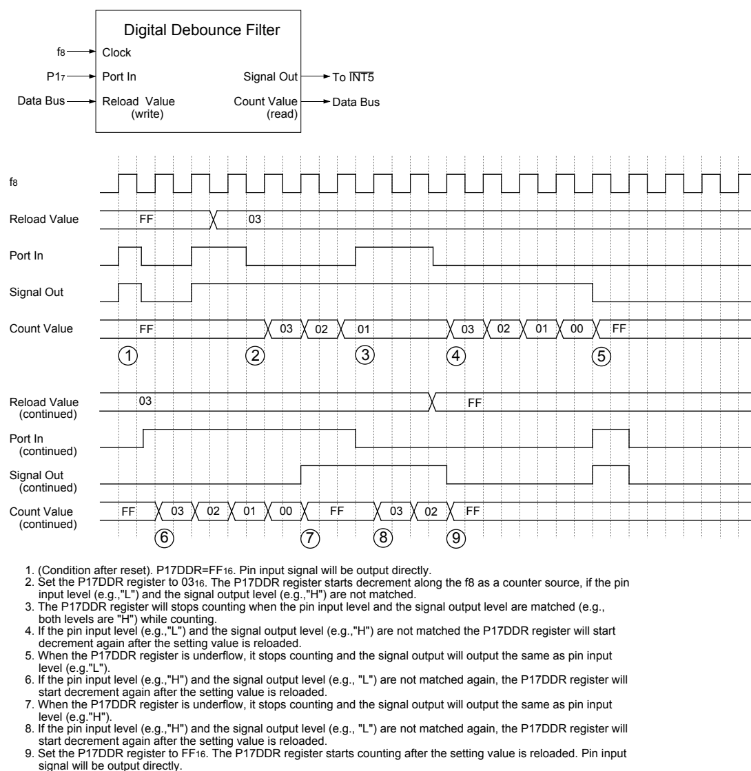
Figure 19.12 Functioning of Digital Debounce Filter
