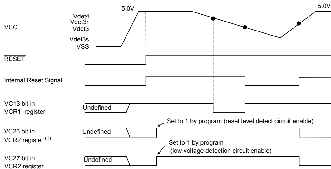
Figure 5.6 D4INT Register
