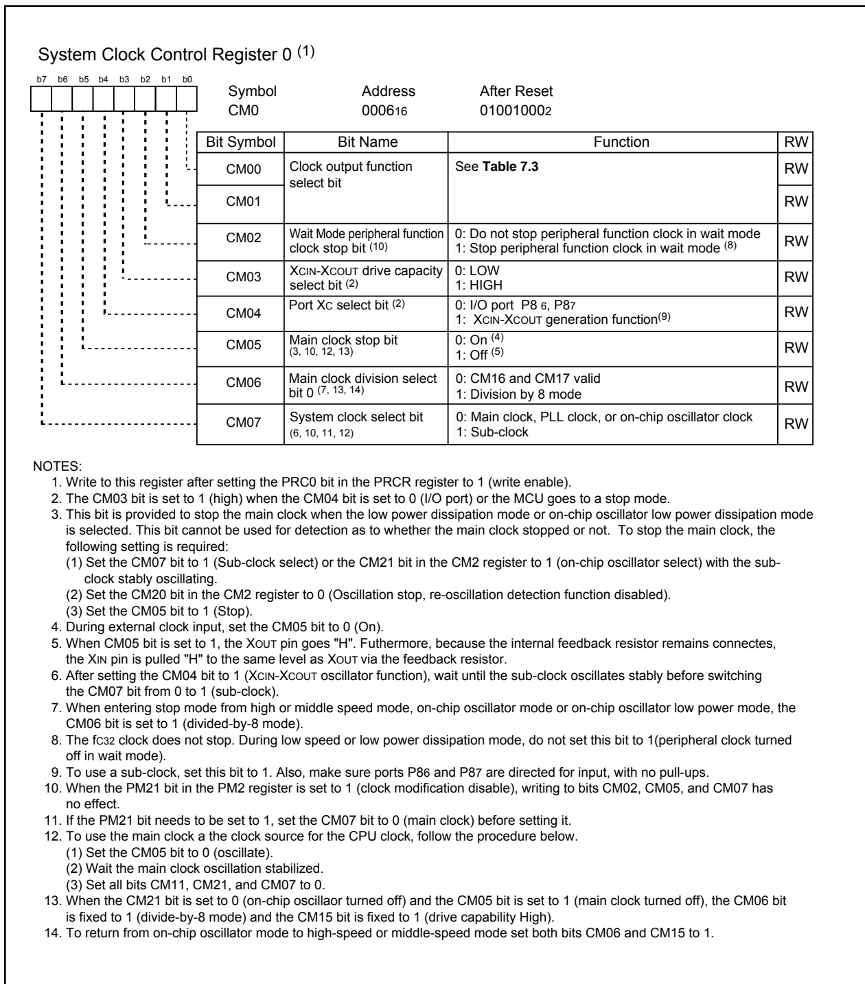
Figure 7.2 CM0 Register
