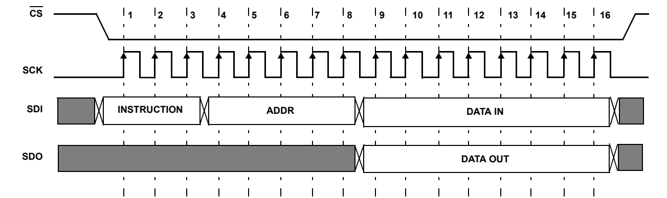
FIGURE 31. TWO BYTE READ INSTRUCTION
