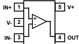
ISL28130 (5 LD SC-70) TOP VIEW
