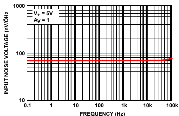
FIGURE 43. SIMULATED INPUT NOISE VOLTAGE DENSITY vs FREQUENCY
