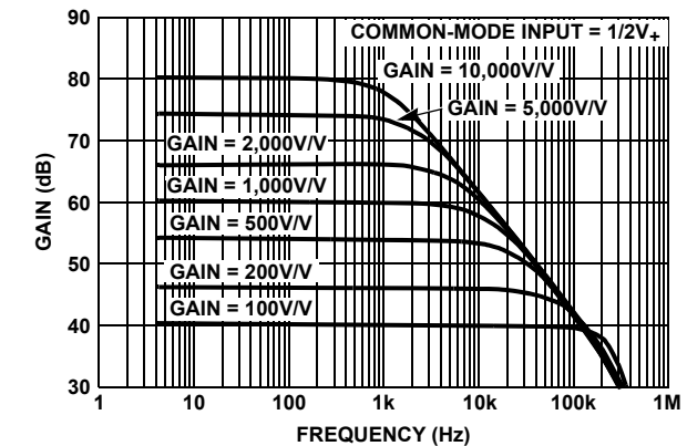
FIGURE 3. ISL28270, ISL28470 FREQUENCY RESPONSE vs CLOSED LOOP GAIN. V_+ = 5V , V_{CM} = 1/2V_+
