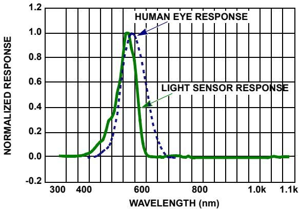
FIGURE 3. SPECTRAL RESPONSE
