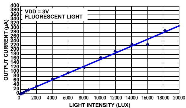
FIGURE 6. OUTPUT CURRENT vs LIGHT INTENSITY
