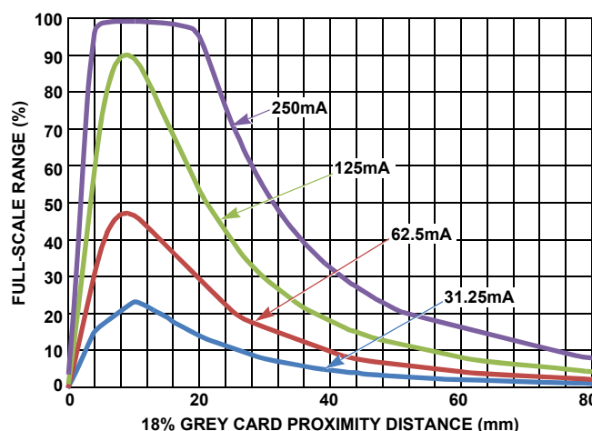
FIGURE 2. PROXIMITY SENSITIVITY
