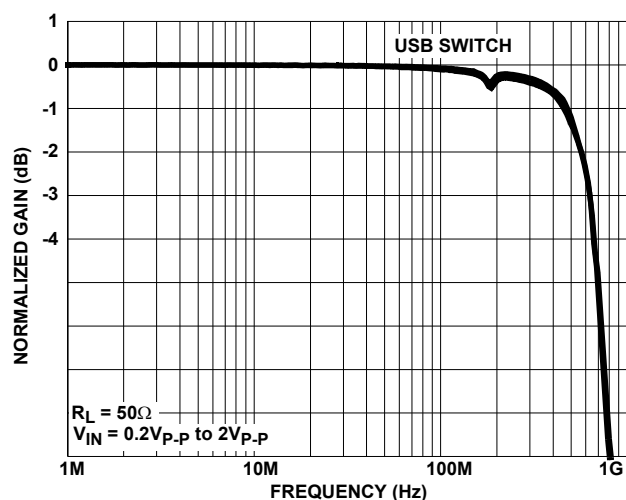
FIGURE 13. FREQUENCY RESPONSE
