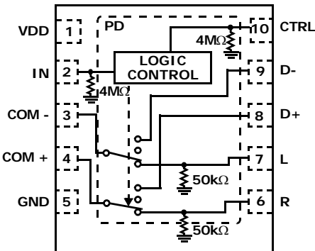
ISL54209 (10 LD 3.0mmx3.0mm TDFN) TOP VIEW
