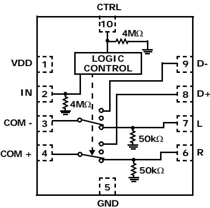
ISL54209 (10 LD 2.1mmx1.6mm \mu TQFN) TOP VIEW
