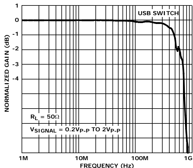
FIGURE 14. FREQUENCY RESPONSE
