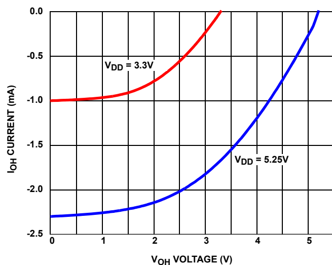
FIGURE 19. I OH vs V OH vs V DD for \overline{\text{INT}}
