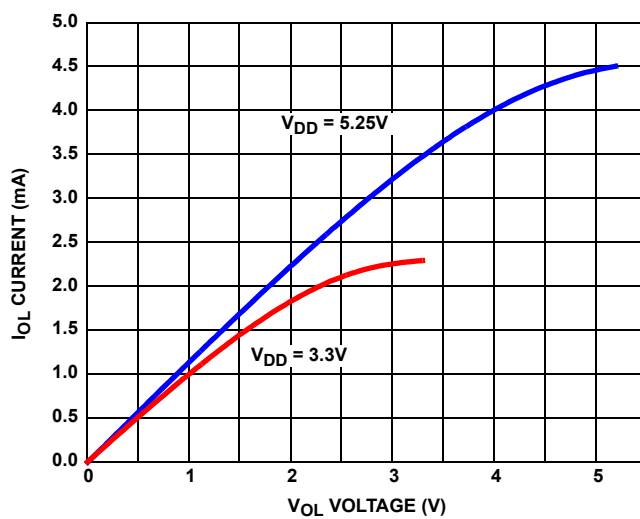
FIGURE 20. I OL vs V OL vs V DD for \overline{\text{INT}}
