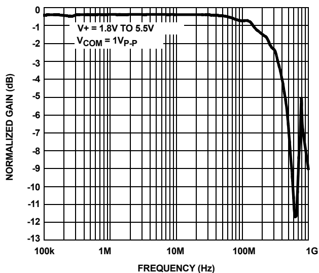
FIGURE 17. FREQUENCY RESPONSE
