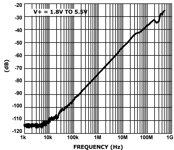
FIGURE 18. OFF-ISOLATION
