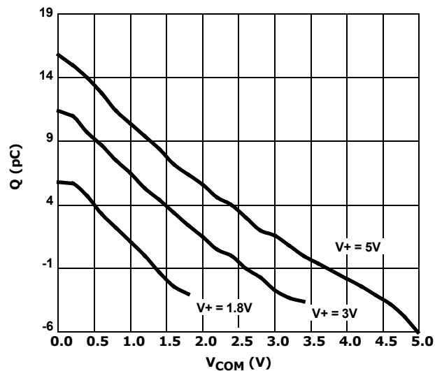
FIGURE 19. CHARGE INJECTION vs SWITCH VOLTAGE
