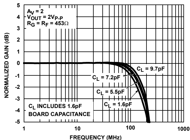
FIGURE 4. LARGE SIGNAL GAIN vs FREQUENCY vs C_L
