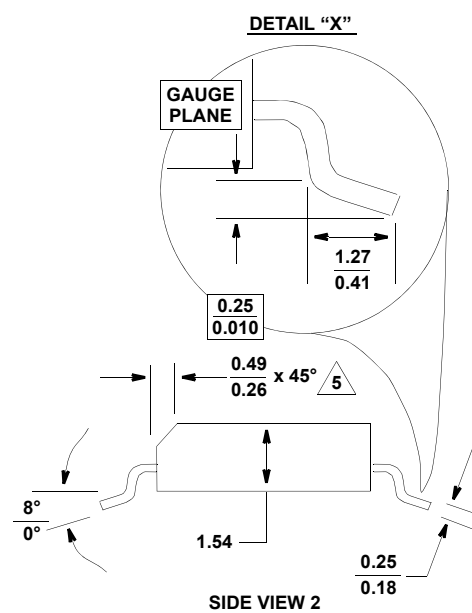
SIDE VIEW 2
