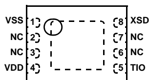
ISL6296 (8 LD 2X3 TDFN) TOP VIEW
