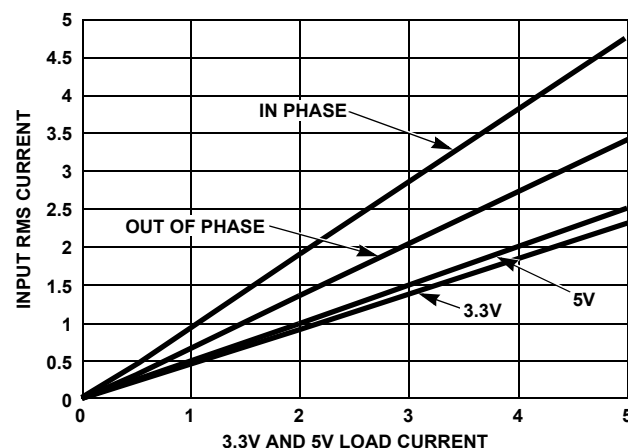
FIGURE 22. INPUT RMS CURRENT vs LOAD
