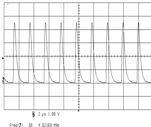
FIGURE 18. SYNC WAVEFORM
