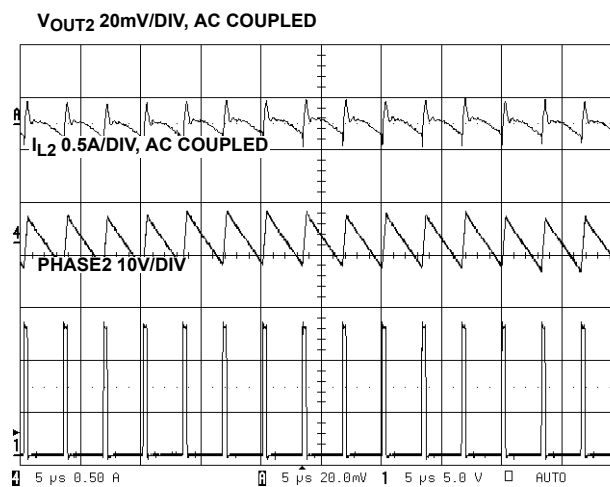
FIGURE 6. PWM2 WAVEFORMS
