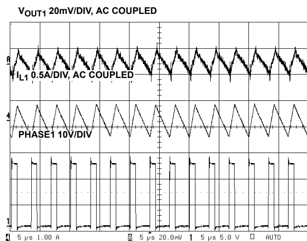
FIGURE 5. PWM1 WAVEFORMS
