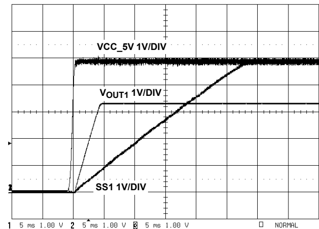
FIGURE 13. SOFT-START OPERATION
