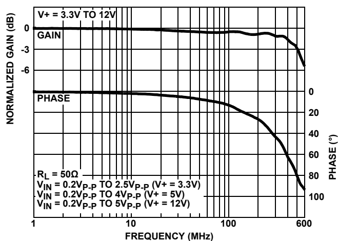
FIGURE 16. FREQUENCY RESPONSE
