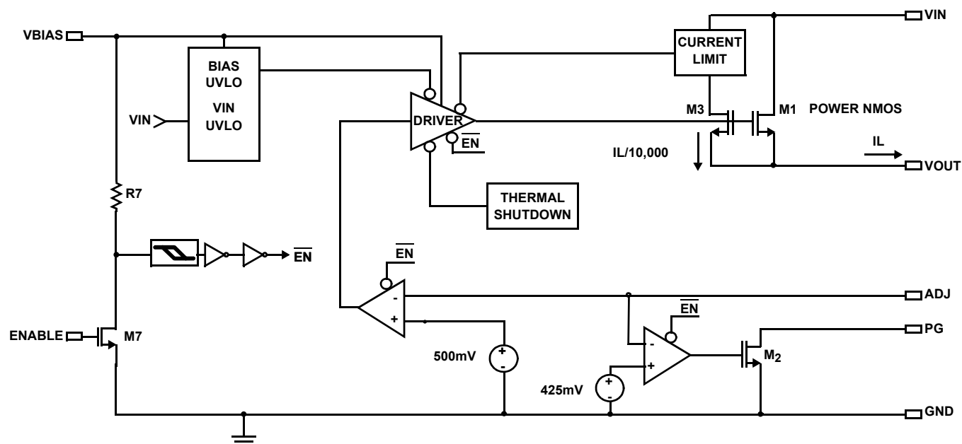
FIGURE 5. BLOCK DIAGRAM
