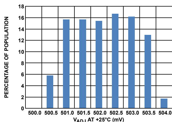
FIGURE 7. V_{ADJ} DISTRIBUTION
