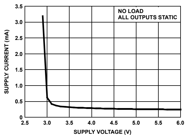
FIGURE 10. SUPPLY CURRENT vs SUPPLY VOLTAGE
