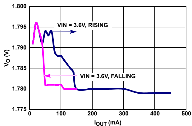
FIGURE 4. OUTPUT VOLTAGE vs LOAD CURRENT (ISL9103, V_{O\_NOMINAL} = 1.8\text{V} )
