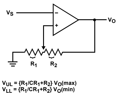
COMPARATOR WITH HYSTERITIS
