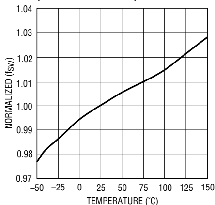
f_{SW} vs Temperature (Measured at 1MHz)
