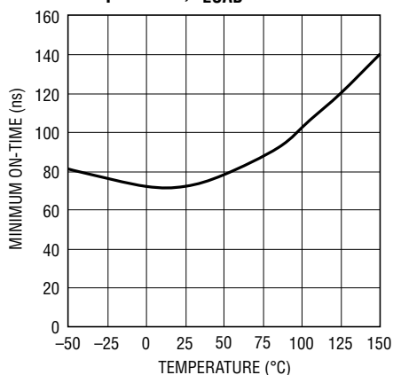
Minimum On-Time vs Temperature, I_{LOAD} = 0.3A
