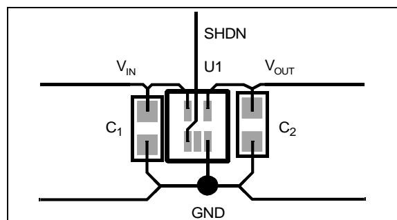
FIGURE 5-1: Suggested layout
