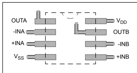
FIGURE 4-10: Recommended Layout.
