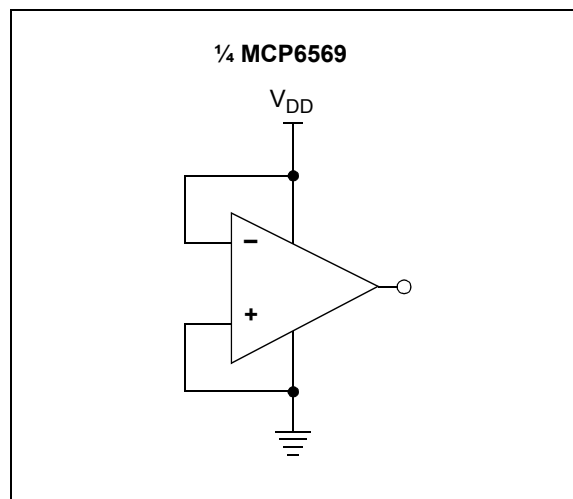
FIGURE 4-11: Unused Comparators.
