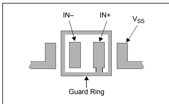
FIGURE 4-9: Example Guard Ring Layout for Inverting Circuit.
