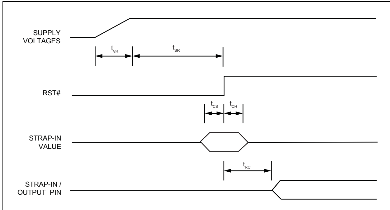
FIGURE 7-10: POWER-UP/RESET TIMING
