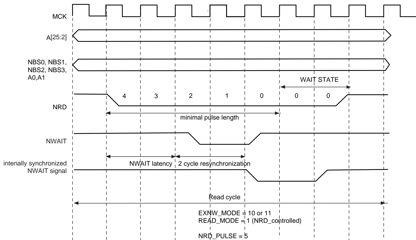
Figure 19-30. NWAIT Latency
