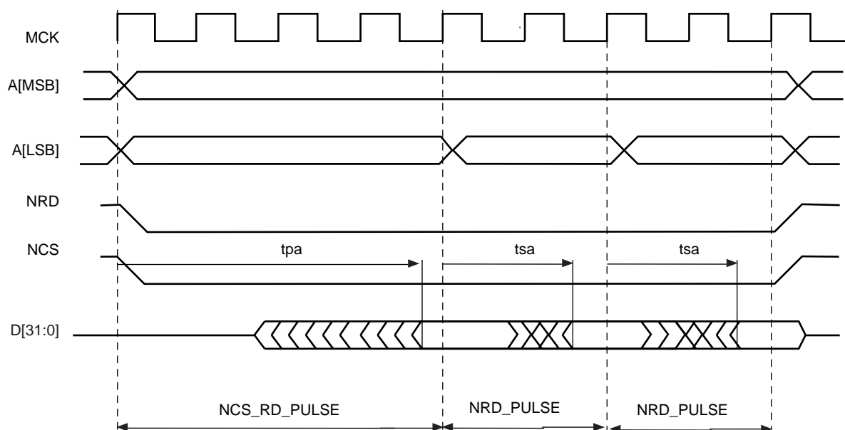
Figure 19-34. Page Mode Read Protocol (Address MSB and LSB are defined in Table 19-6 )
