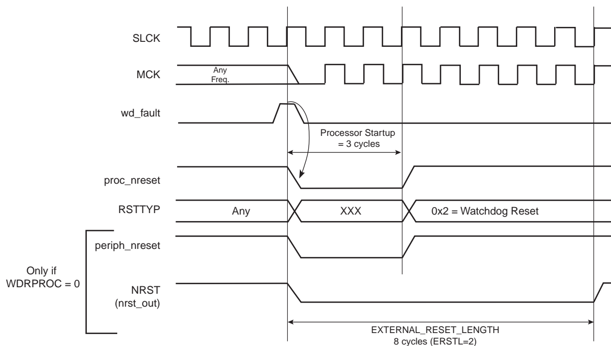
Figure 12-8. Watchdog Reset
