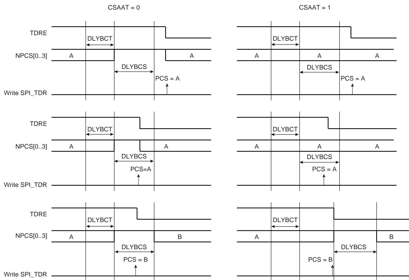
Figure 28-8. Peripheral Deselection
