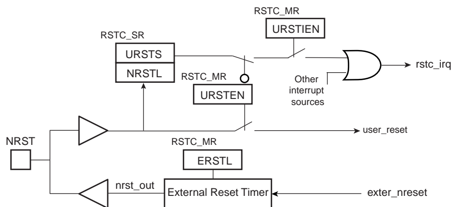
Figure 12-2. NRST Manager
