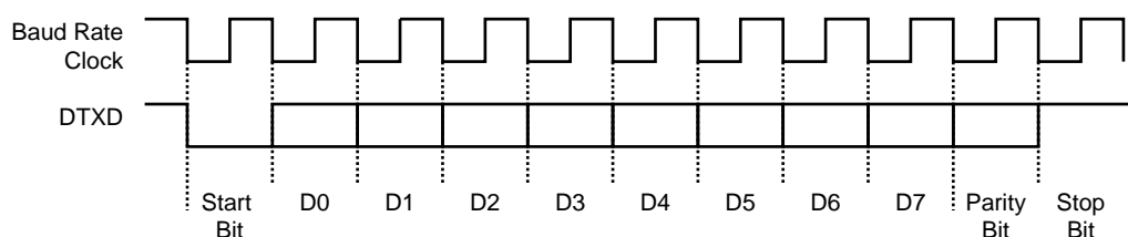
Figure 26-10. Character Transmission
