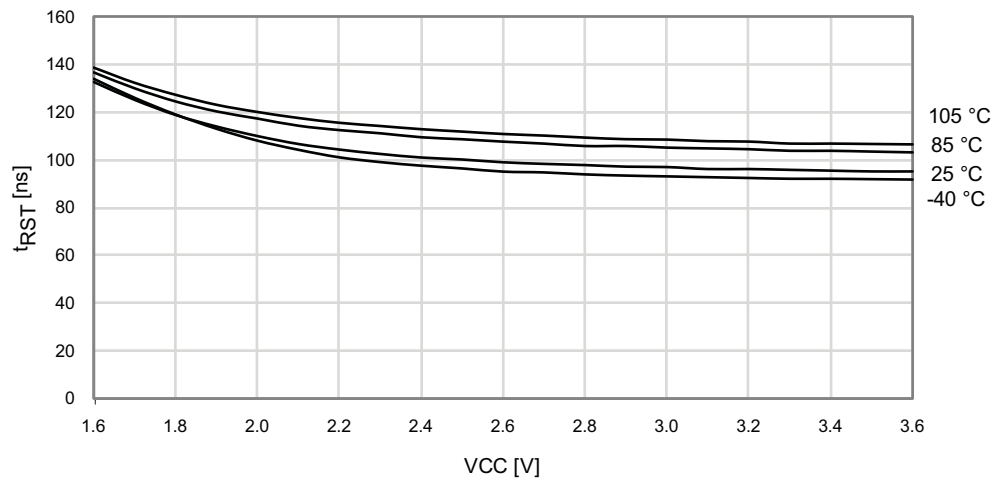
Figure 34-190. Minimum Reset Pin Pulse Width vs. V CC
