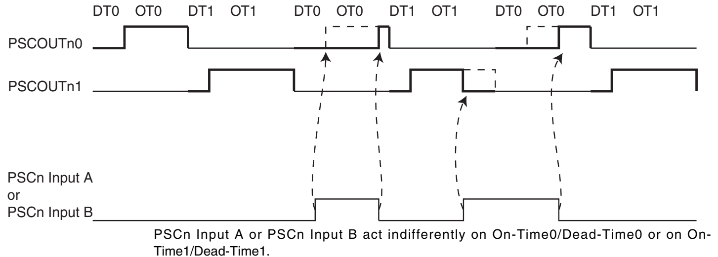
Figure 12-29. PSC behavior versus PSCn Input A or Input B in Fault Mode 4.
