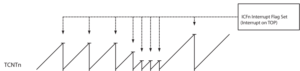
Figure 11-5. CTC mode, timing diagram.
