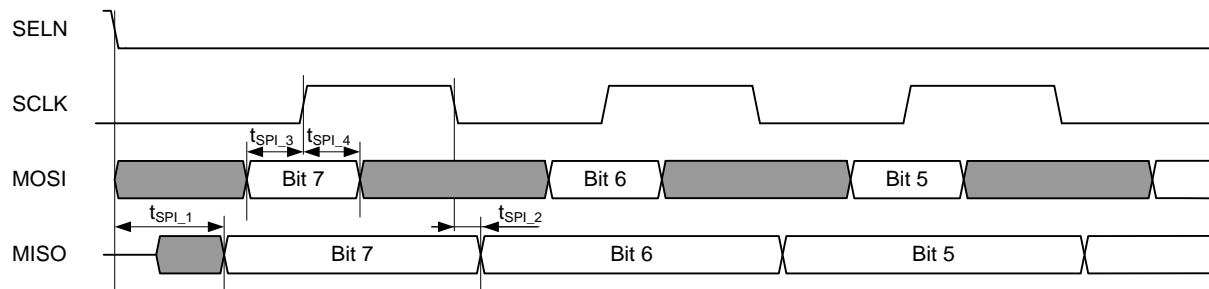
Figure 4-7. SPI Timing, Definition of Timing Parameters t_{SPI\_1} to t_{SPI\_4} .
