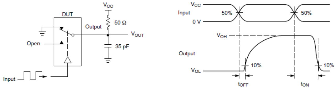
Figure 7. t_{ON} / t_{OFF}
