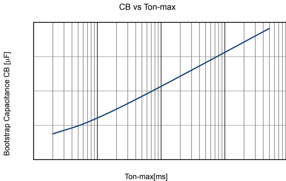
Fig.14 Ton-max vs CB characteristic
