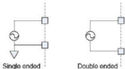
Figure 3: Single and Double Ended Line Inputs
