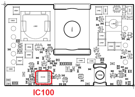
Fig 17: Conformal coating will be applied over IC100 for SQE48T40050 NGALG to pass Telcordia GR-63-CORE Mixed Flow Gas Test
