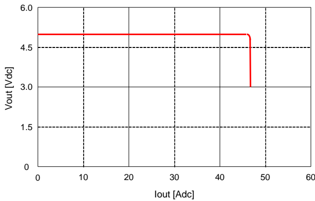
Fig. 15: Output voltage vs. load current showing limit point and converter shutdown point. Input voltage has almost no effect on current limit characteristic
