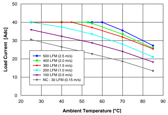
Fig. 2: Available load current vs. ambient air temperature and airflow rates for converter with G height pins mounted horizontally with air flowing from pin 1 to pin 3, MOSFET temperature \le 120^\circ\text{C} , V_{in} = 48\text{ V}
