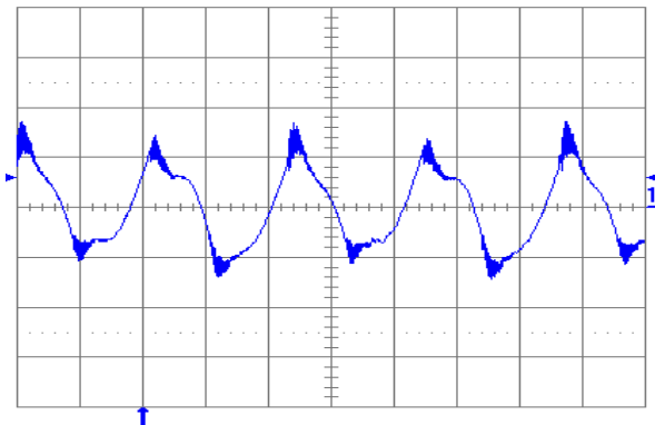
Fig. 11: Output voltage ripple (20 mV/div.) at full rated load current into a resistive load with C_o = 10\text{ }\mu\text{F} tantalum + 1 \mu\text{F} ceramic and V_{in} = 48\text{ V} . Time scale: 1 \mu\text{s} /div.
