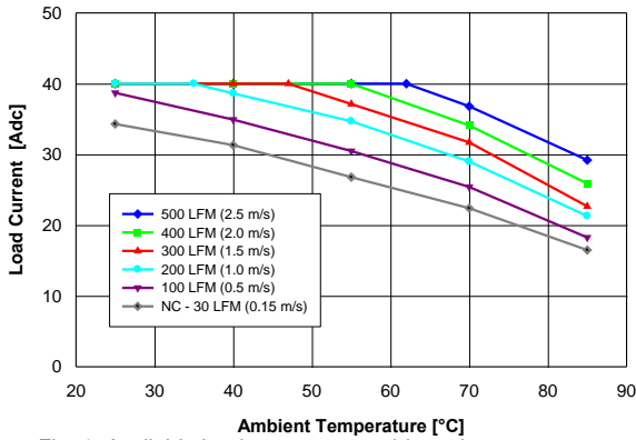
Fig. 1: Available load current vs. ambient air temperature and airflow rates for converter with G height pins mounted vertically with air flowing from pin 1 to pin 3, MOSFET temperature \le 120^\circ\text{C} , V_{in} = 48\text{ V} Note: NC – Natural convection
