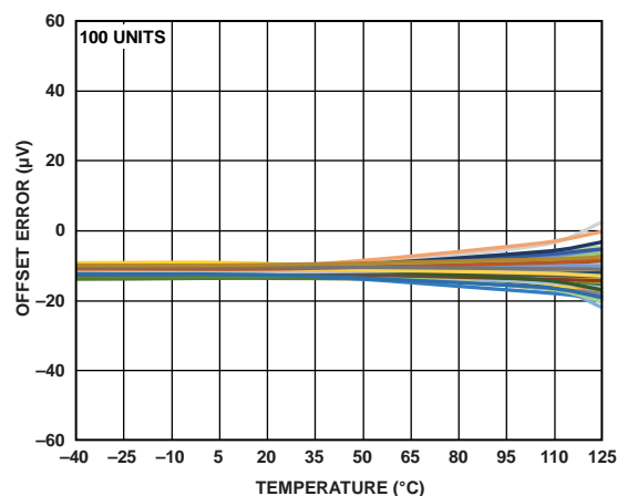
Figure 20. Input Referred Offset Error vs. Temperature (Gain = 16, Mid Power Mode)
