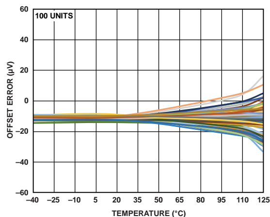
Figure 21. Input Referred Offset Error vs. Temperature (Gain = 16, Low Power Mode)
