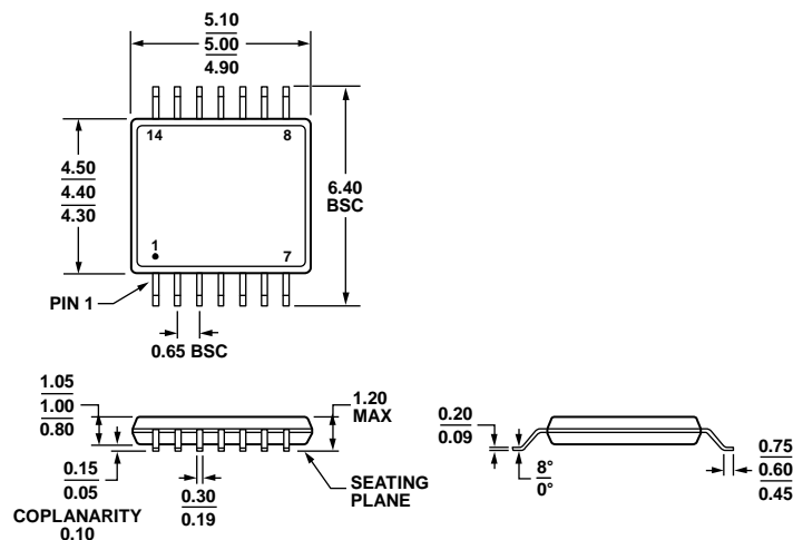
COMPLIANT TO JEDEC STANDARDS MO-153-AB-1 Figure 18. 14-Lead Thin Shrink Small Outline Package [TSSOP] (RU-14) Dimensions shown in millimeters
